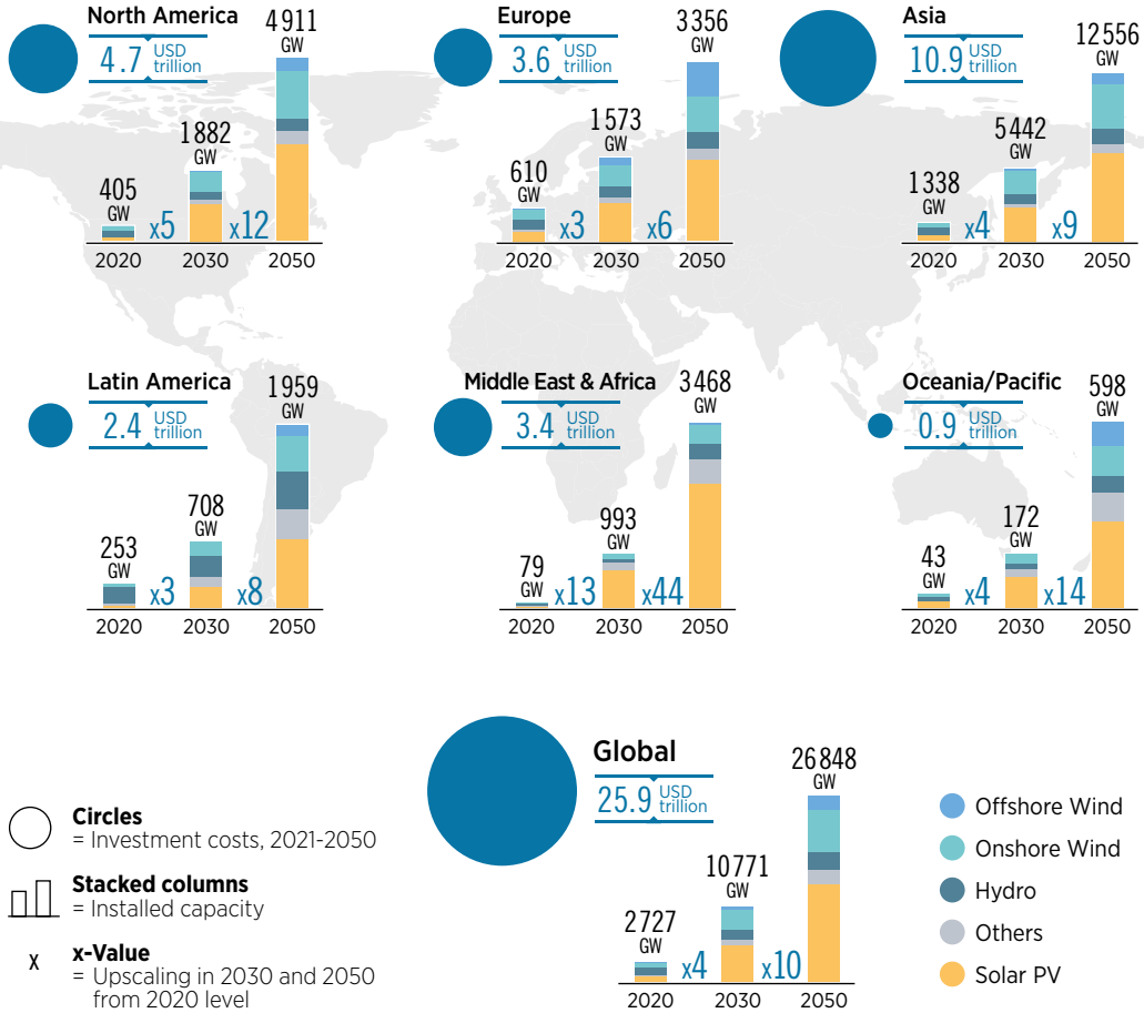
FIGURE 2.4 Regional distribution of total installed capacity (GW) in 2020, 2030, 2050 and cumulative investments (USD trillion) of renewables for power generation in the 1.5°C Scenario across regions, 2021-2050
